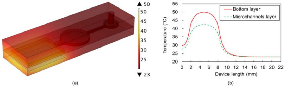
Figure 3. Simulation results. (a) 3D model of the micropump showing the temperature distribution profile of the device. (b) Temperature distribution profile along the bottom and microchannels layers of the device
