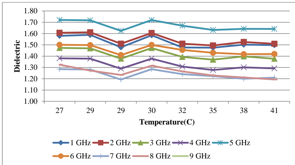
Figure 7. Dielectric permittivity versus temperature
