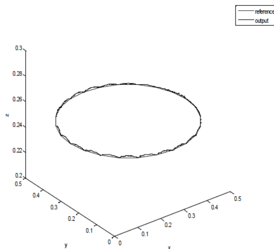
Figure 8. Inverse dynamic tracking control
