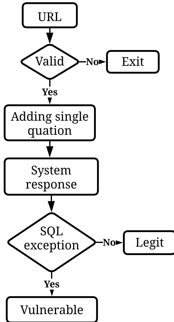
Fig. 1: SQLi vulnerability check of a web application.
