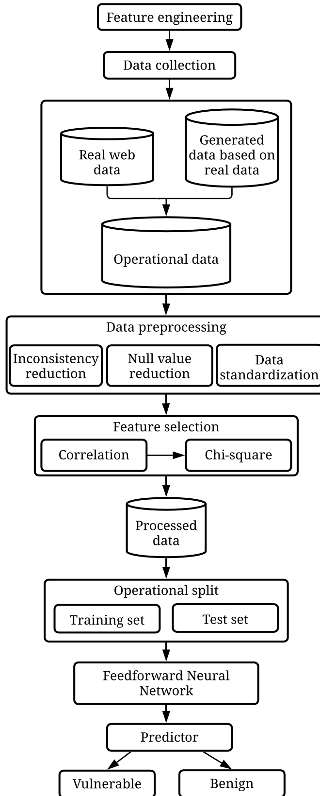
Fig. 2: Proposed model of SQLi vulnerability detection.
