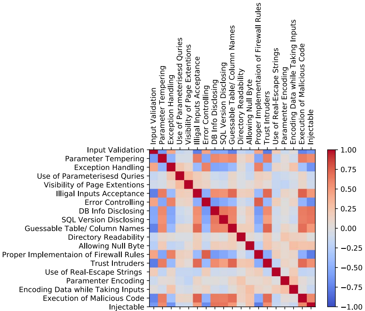
Fig. 3: Visualization of correlated features.
