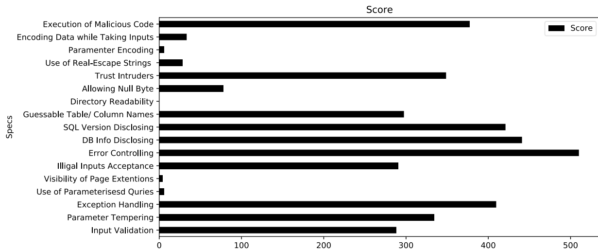
Fig. 4: Plot describing chi-square level of significance. Each plot refers to a particular attribute and shows how important they are to the classification operation.
