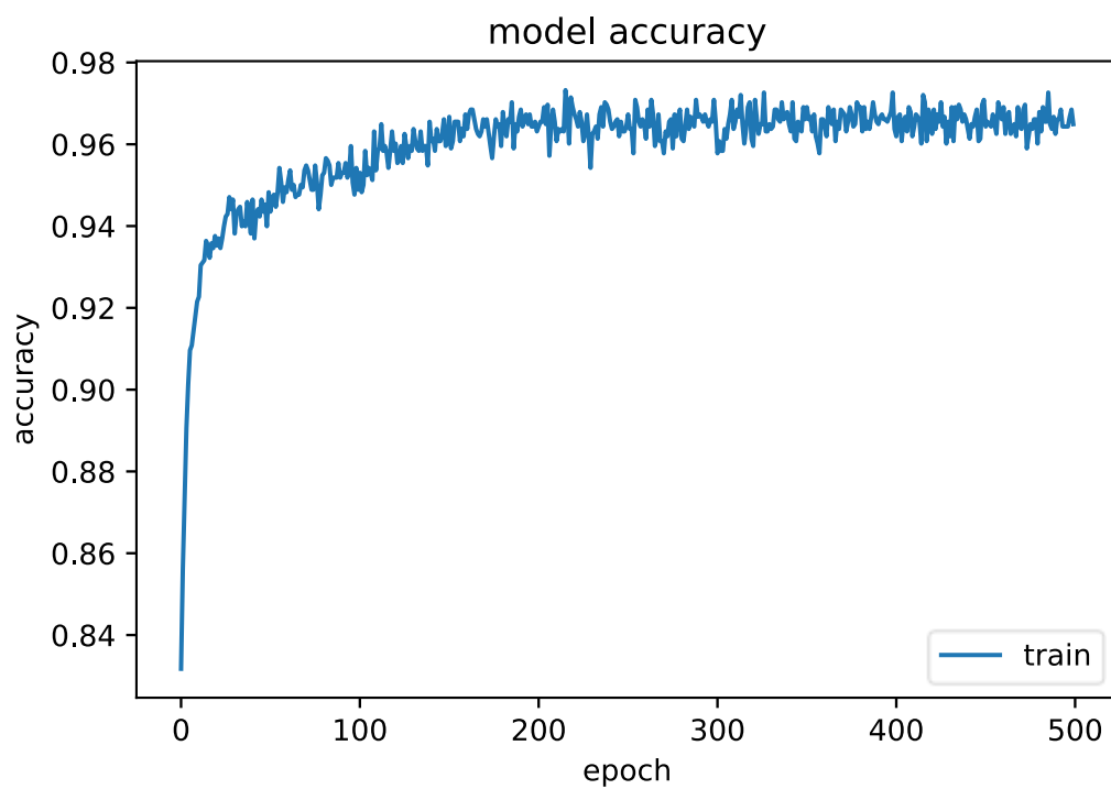
Fig. 5: Adeptness of model at gaining accuracy.
