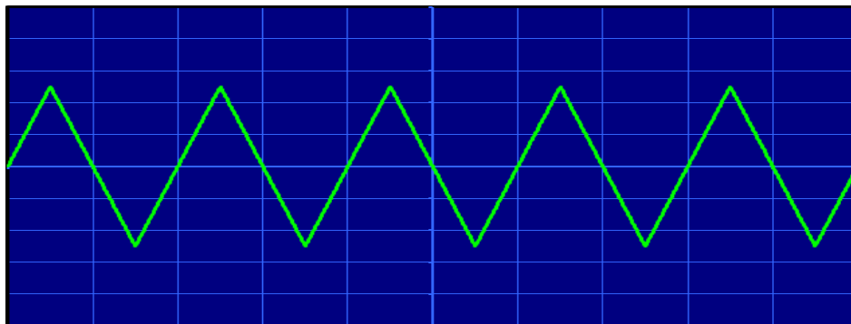
Figure 2. Triangular Wave, Frequency 2500 Hz, Amplitude 10 V.
