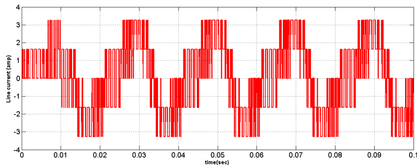
Figure 11. Waveform of phase output line current of six- pulse VSI with Resistive load with PWM triggering.
