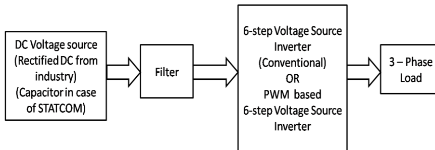
Figure 1. Block diagram of VSI connected to 3- Phase load
