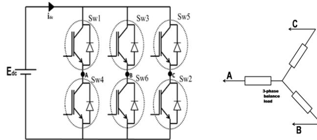
Figure 3. Basic structure of three-phase six-pulse voltage source inverter.
