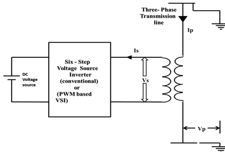
Figure 2. Block diagram of VCI connected as a element of STATCOM.
