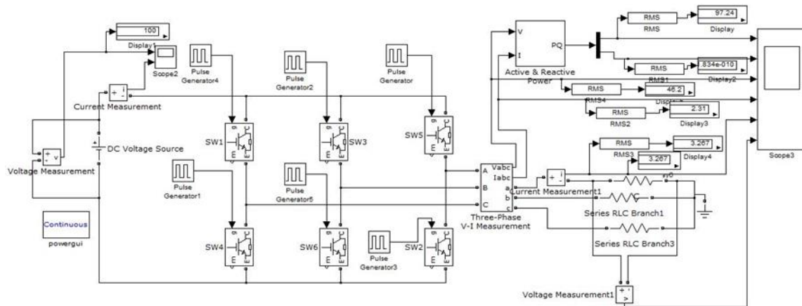
Figure 5. Simulink model of six pulse VSI with resistive load
