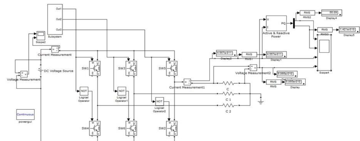
Figure 6. Simulation Diagram of 6-pulse PWM based VSI with R load
