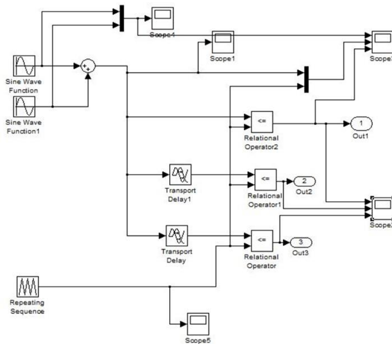
Figure 7. Simulation Diagram of PWM generator
