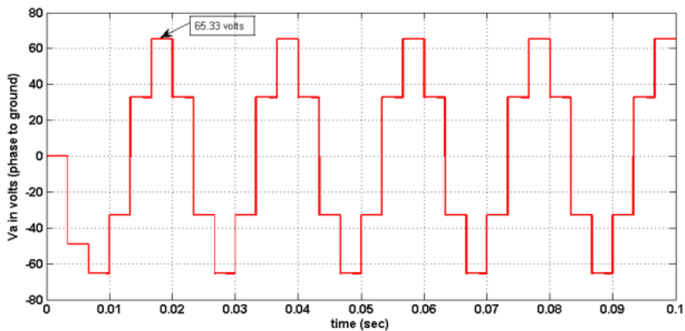
Figure 8. Voltage response of six pulse VSI based STATCOM using conventional triggering
