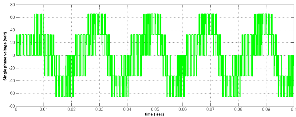
Figure 10. Waveform of phase voltage of six- pulse VSI with Resistive load with PWM triggering.
