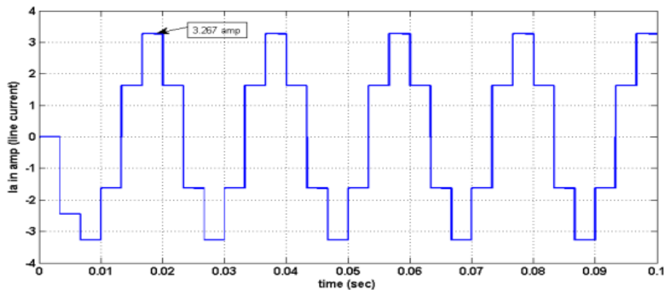
Figure 9. Current response of six pulse VSI based STATCOM using conventional triggering
