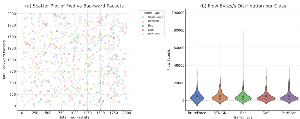
Figure 4. Exploratory Visualizations of CIC-IDS2017 Dataset Showing (a) Packet Distribution Across Forward and Backward Flows by Traffic Type, and (b) Flow Bytes per Second Distribution Across Different Traffic Classes
