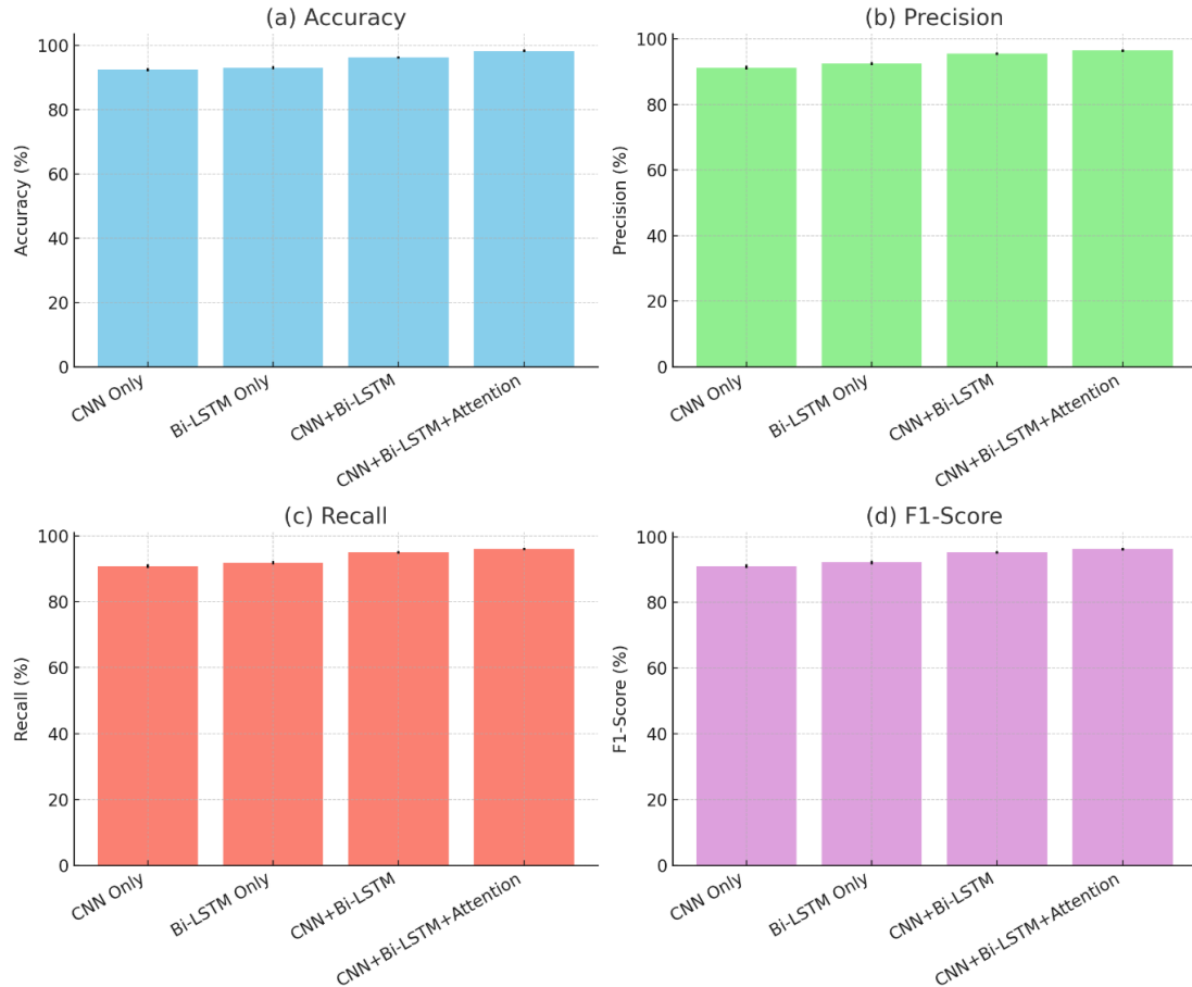
Figure 10. Ablation Study Results of IntruNet-Hybrid On CIC-IDS2017 Dataset with Standard Deviations
