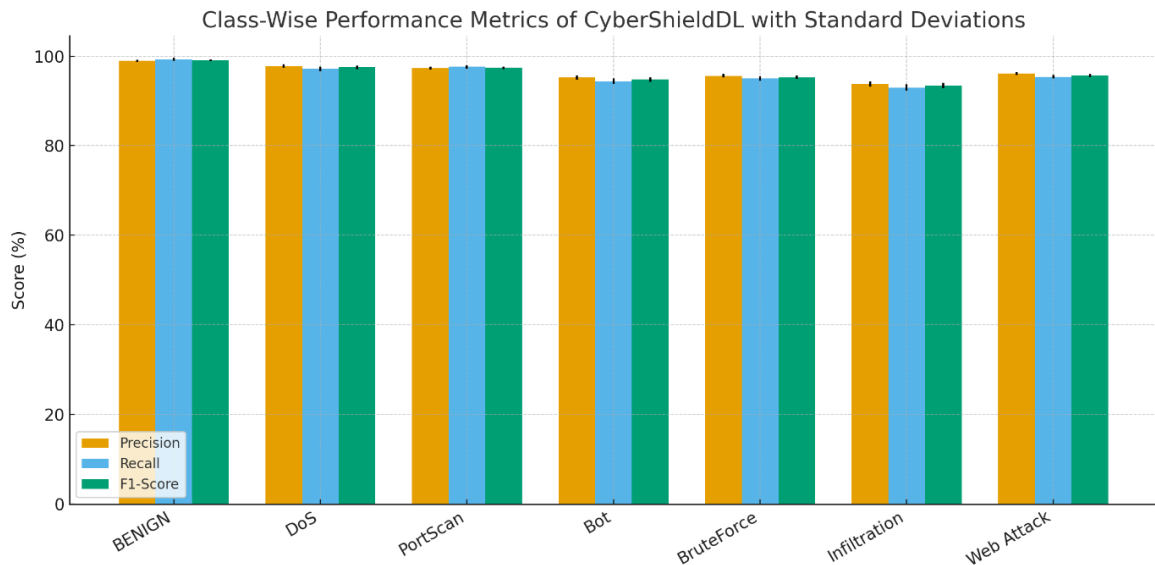
Figure 5. Class-Wise Performance Metrics of CyberShieldDL On CIC-IDS2017 Dataset with Standard Deviations
