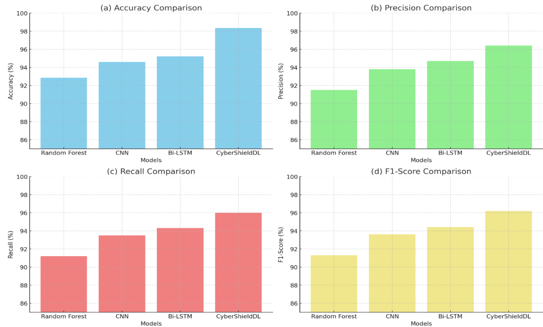
Figure 6. Performance Comparison of CyberShieldDL With Baseline Models on CIC-IDS2017 Dataset Showing (a) Accuracy, (b) Precision, (c) Recall, and (d) F1-Score Across Different Models
