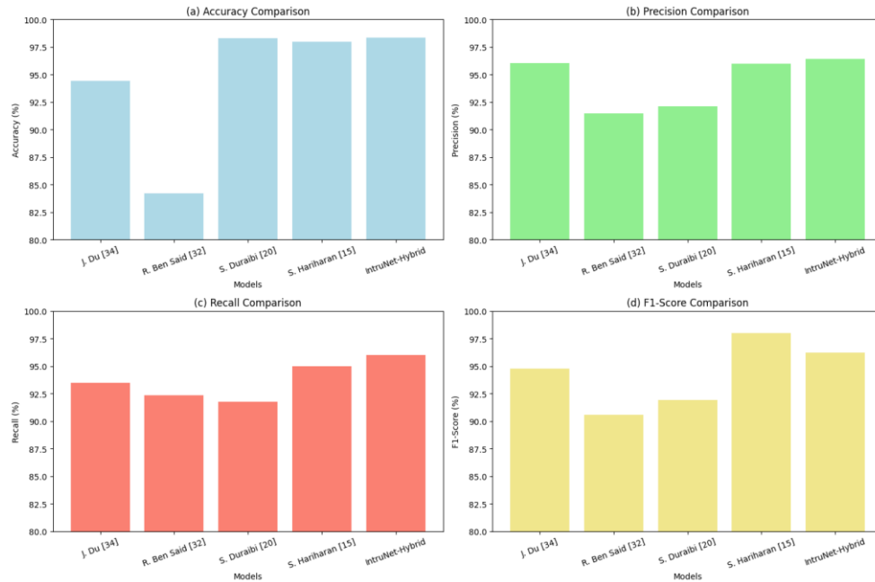
Figure 11. Comparative Performance Analysis of IntruNet-Hybrid and Existing Methods on CIC-IDS2017 Dataset
