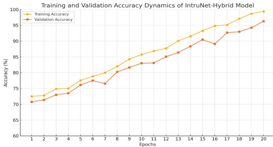
Figure 7. Training and Validation Accuracy Dynamics of the IntruNet-Hybrid Model Across Epochs on the CIC-IDS2017 Dataset
