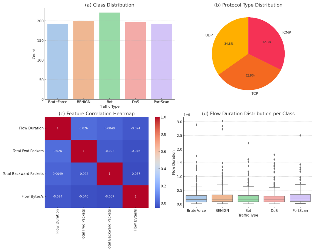
Figure 3. Exploratory Data Analysis of CIC-IDS2017 Dataset Showing (a) Class Distribution, (b) Protocol Type Usage, (c) Feature Correlations, and (d) Flow Duration Across Traffic Classes
