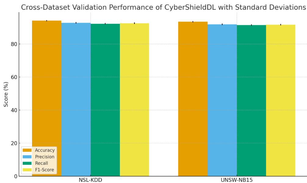
Figure 9. Cross-Dataset Validation Performance of CyberShieldDL On NSL-KDD And UNSW-NB15 Datasets with Standard Deviations
