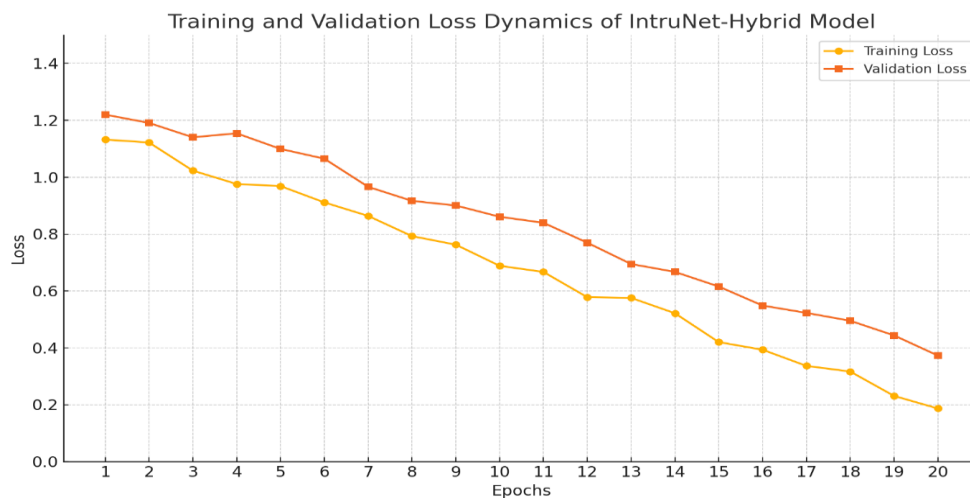
Figure 8. Training and Validation Loss Dynamics of the IntruNet-Hybrid Model Across Epochs on the CIC-IDS2017 Dataset
