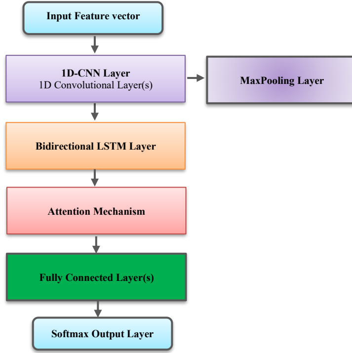
Figure 2. IntruNet-Hybrid Model with CNN, Bi-LSTM, and Attention for Intrusion Classification
