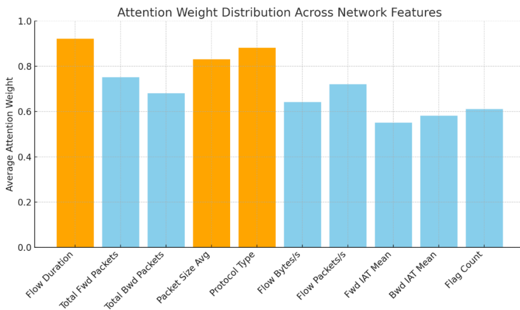
Figure 12. Attention Weight Distribution Across Network Features for Representative Attack Classes
