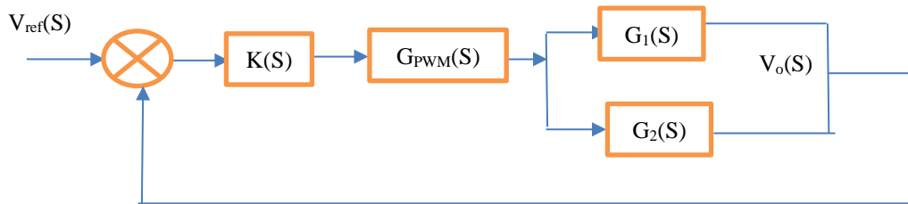
Figure 1. Closed loop controller of the hybrid system
