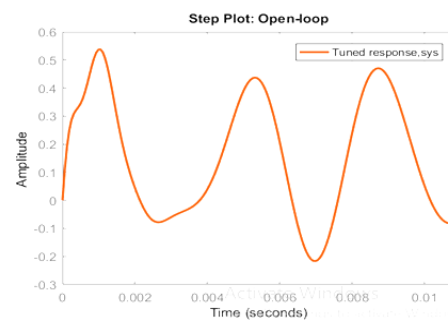
Figure 3. Step response of the system
